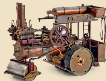
Two-Cylinder Steam Road Roller, c. 1922 Coal-fired boiler. – A very well-constructed and impressive model. Estimate: 2,400 – 3,000 € / 2,800 – 3,500 US$
