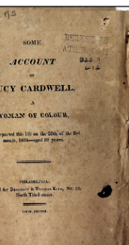
Slave Documents
